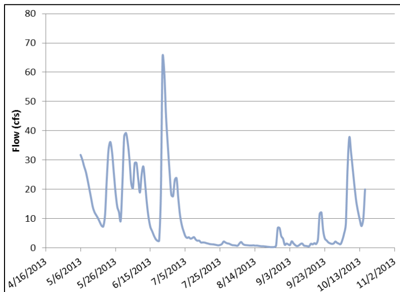
Figure 44. Continuous flow monitoring, Rock Creek (2013)
