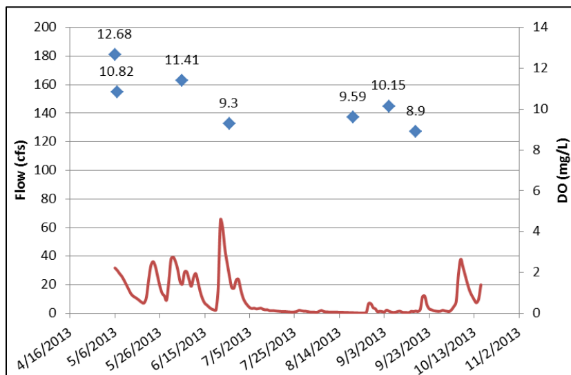
Figure 46. 2013 DO data compared to flow on Rock Creek
