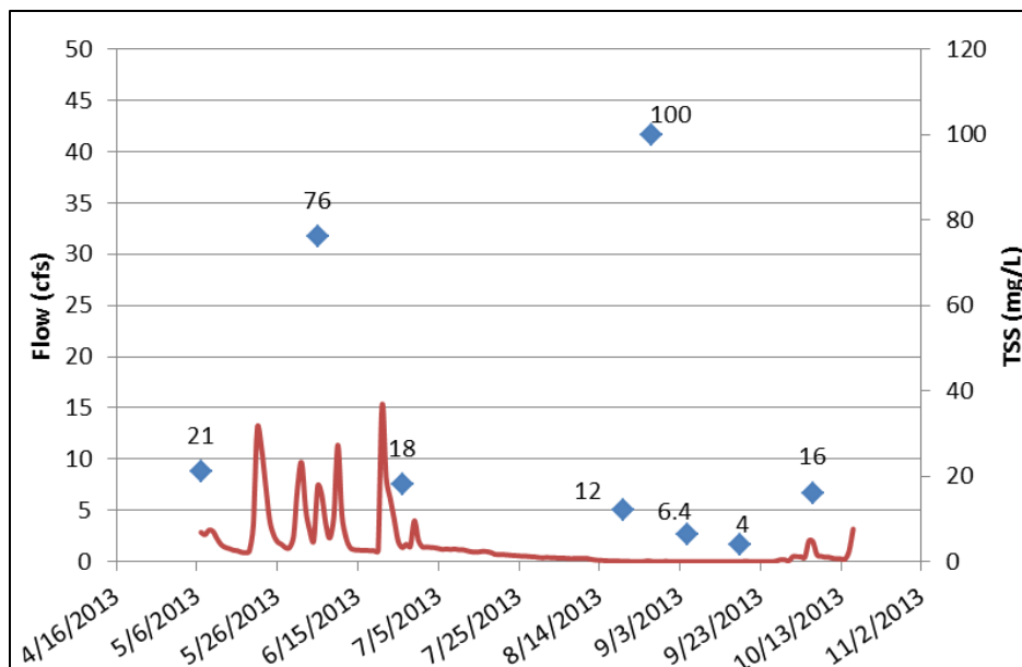
Figure 40. TSS concentrations in Elim Creek, 2013
