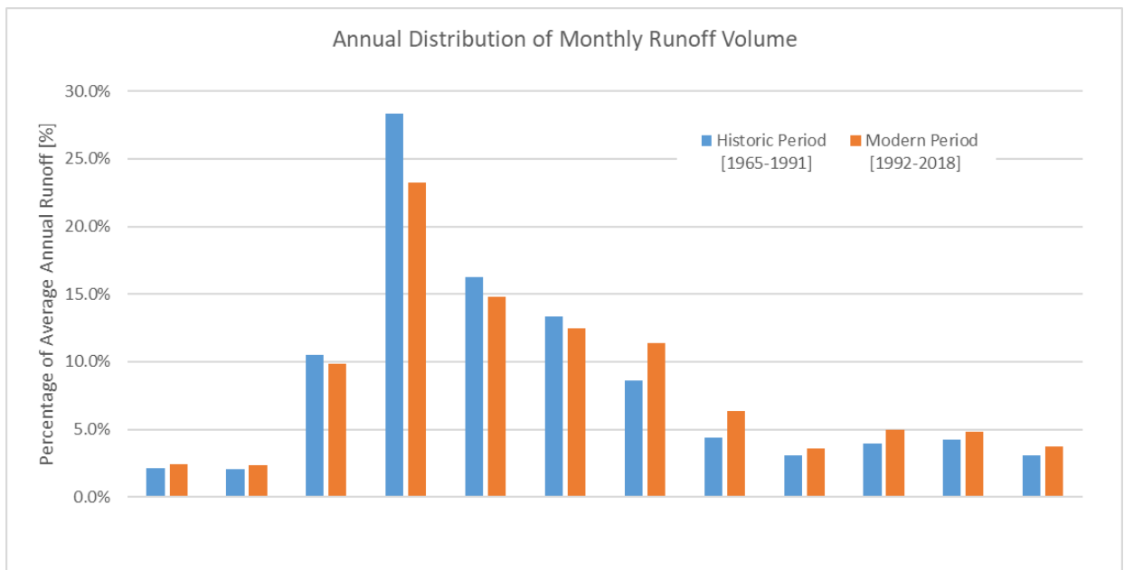
Figure A.4. Annual distribution of average monthly runoff volume as a percentage of annual total volume in the Minnesota River at Montevideo, MN (USGS# 05311000).
