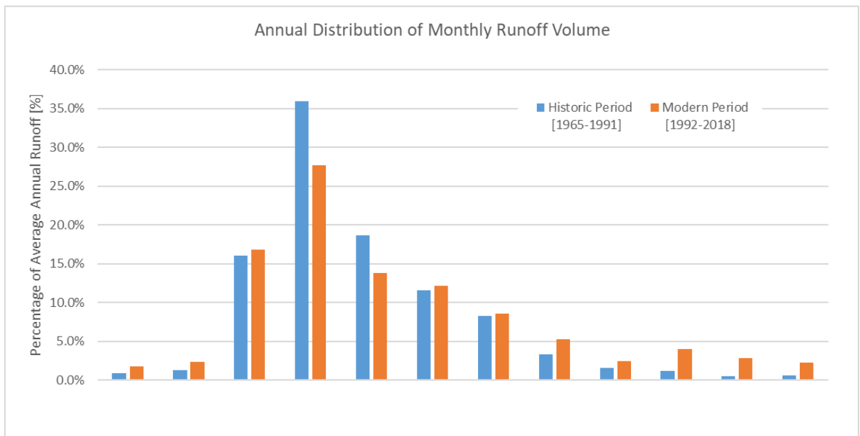
Figure A.4. Annual distribution of average monthly runoff volume as a percentage of annual total volume in the Minnesota River at Ortonville, MN (USGS# 05292000).
