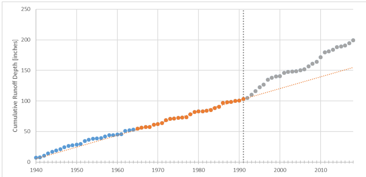
Figure 1. Cumulative streamflow for Whetstone River Near Big Stone City, SD (USGS# 05291000).
