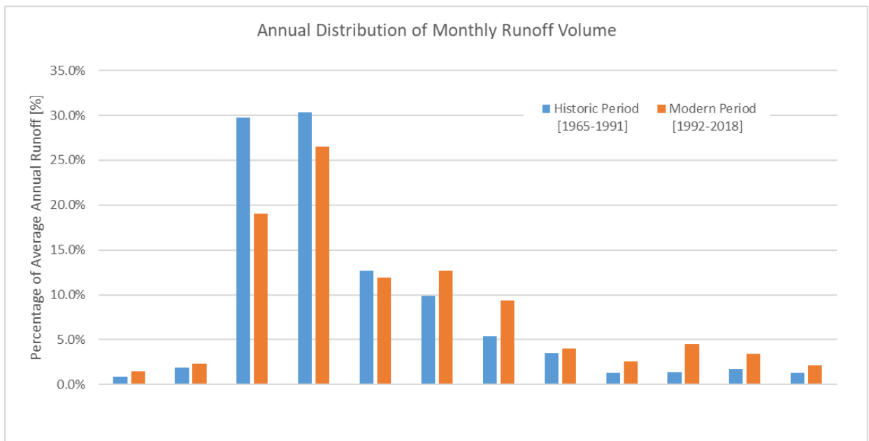
Figure A.4. Annual distribution of average monthly runoff volume as a percentage of annual total volume in the Whetstone River Near Big Stone City, SD (USGS# 05291000).
