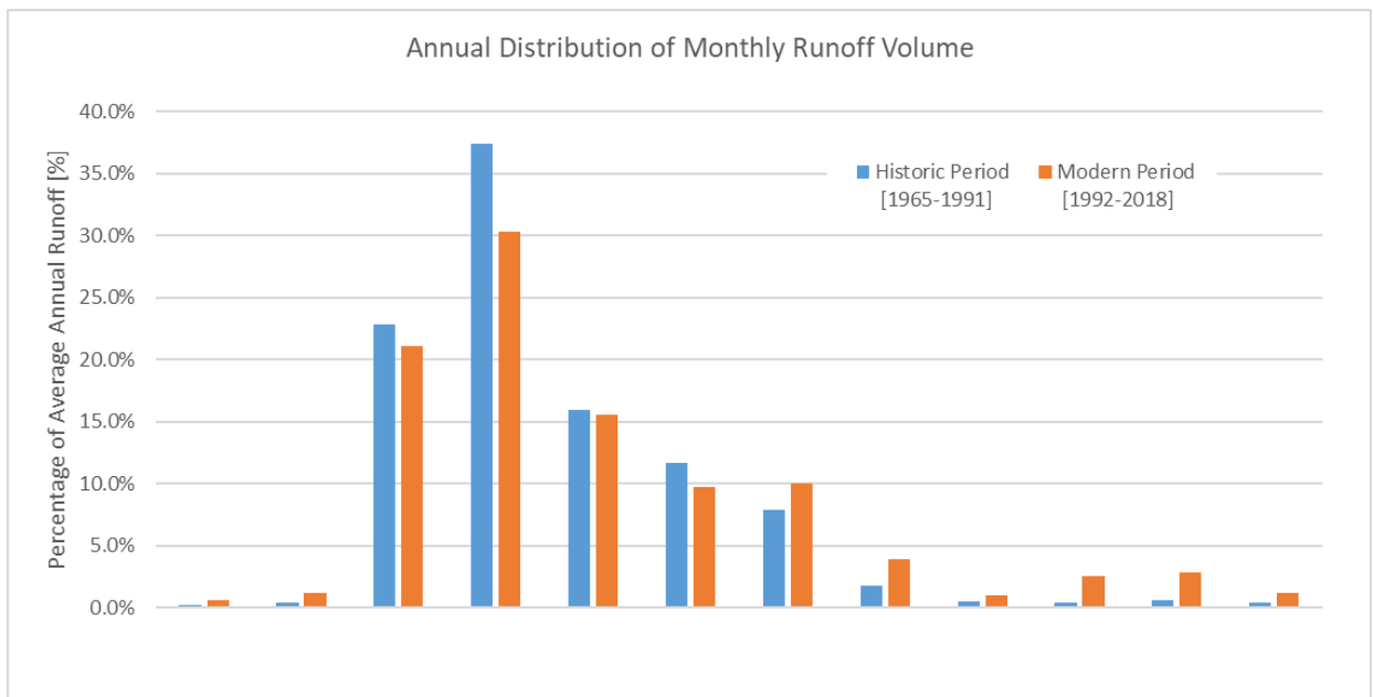
Figure A.4. Annual distribution of average monthly runoff volume as a percentage of annual total volume in the Little Minnesota River near Peever, SD (USGS# 05290000).
