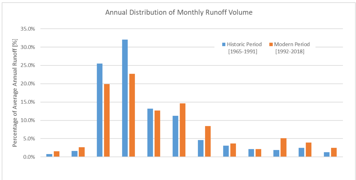
Figure A.4. Annual distribution of average monthly runoff volume as a percentage of annual total volume in the Yellow Bank River near Odessa, MN (USGS# 05293000).
