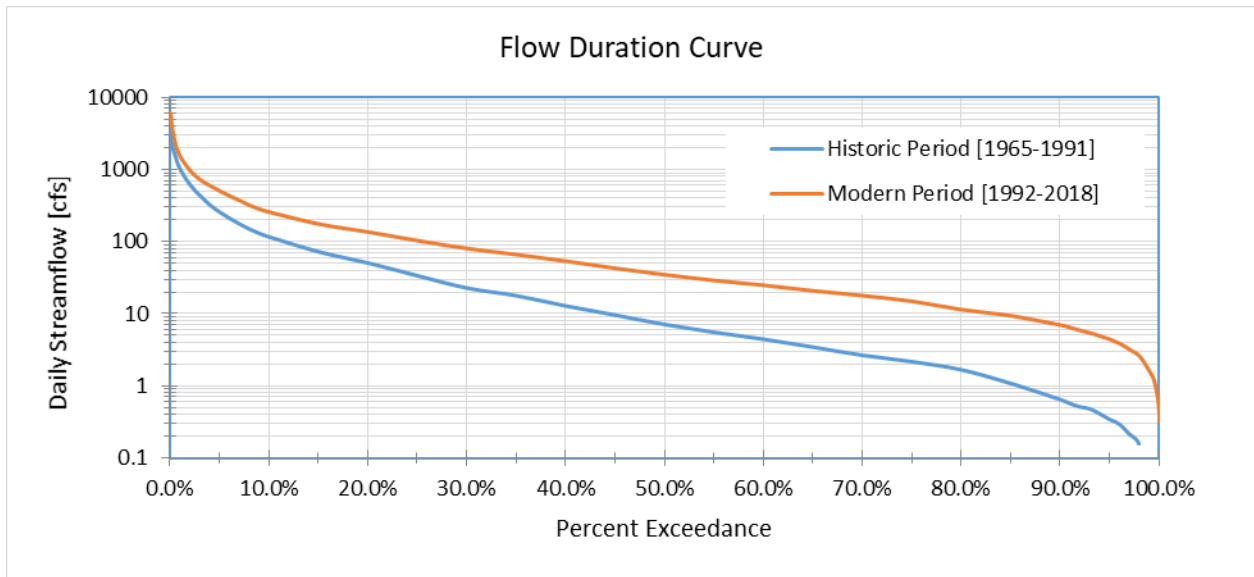
Figure 23. Flow duration curve for Yellow Bank River near Odessa, MN (USGS# 05293000). Comparing two periods, a “historic” benchmark condition (1965-1991) and a modern condition (1992-2018).
