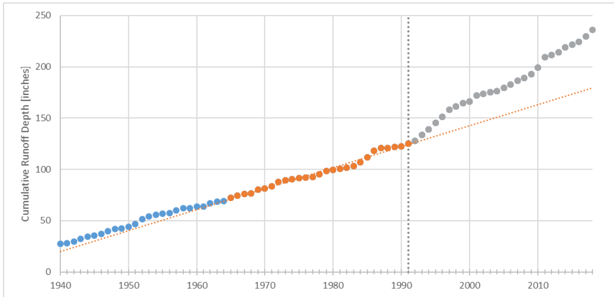
Figure 1. Cumulative streamflow for Minnesota River at Montevideo, MN (USGS# 05311000).
