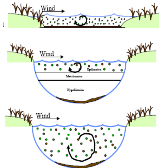
Figure 1. Lake stratification
