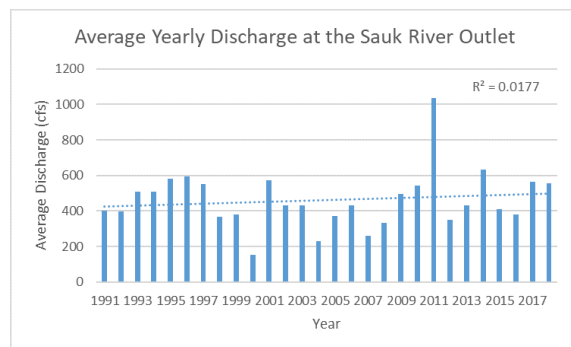
Figure 6. Sauk River annual flow (cfs)
