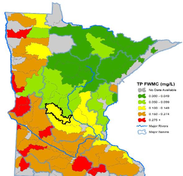
Figure 4. Average total phosphorus flow weighted mean concentrations (FWMC) by major watershed. The Sauk River Watershed is outlined in black.
