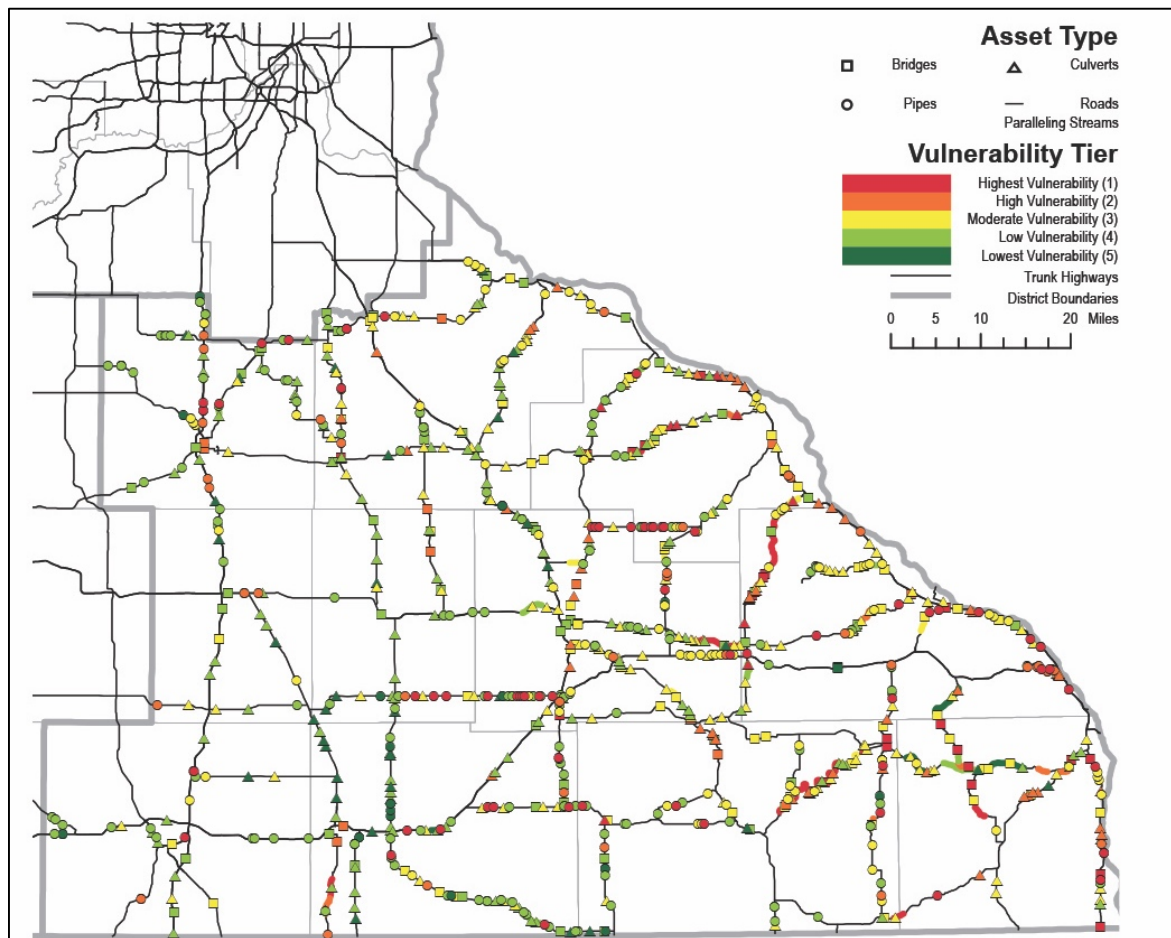
Asset vulnerability to flash flood events in MnDOT District 6. Source: MnDOT
